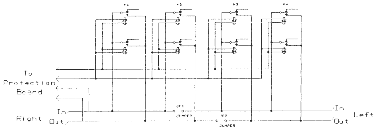
Relay Board
