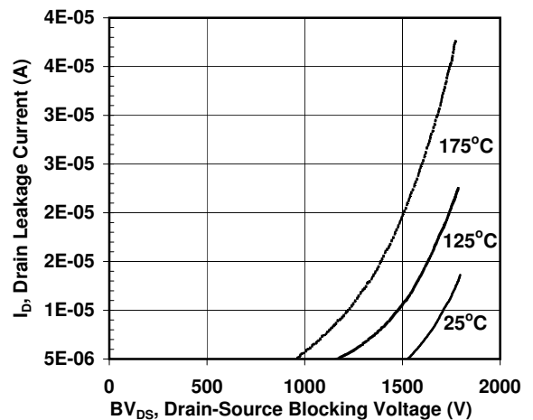
Figure 12. Drain-Source Leakage
