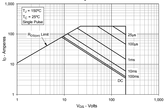
Fig. 15. Forward-Bias Safe Operating Area @ T C = 25°C
