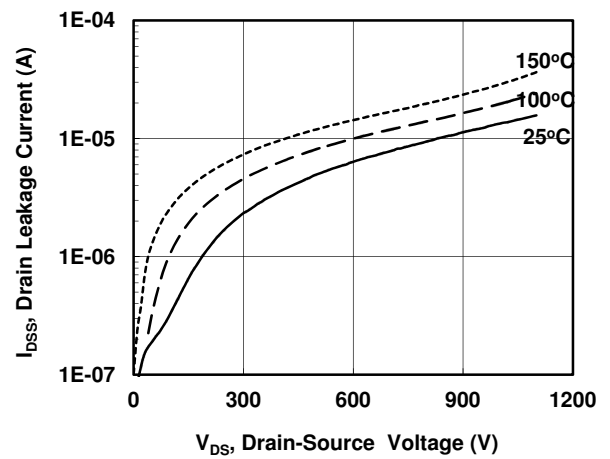
Figure 10. Drain-Source Leakage
