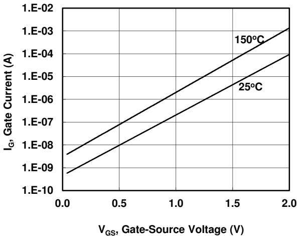
Figure 5. Gate Current
