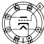
G-5U BOTTOM VIEW
