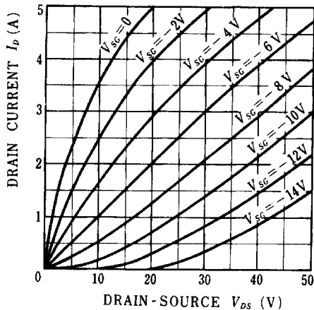
Sample I ( V_p = 22.80V )の静特性
