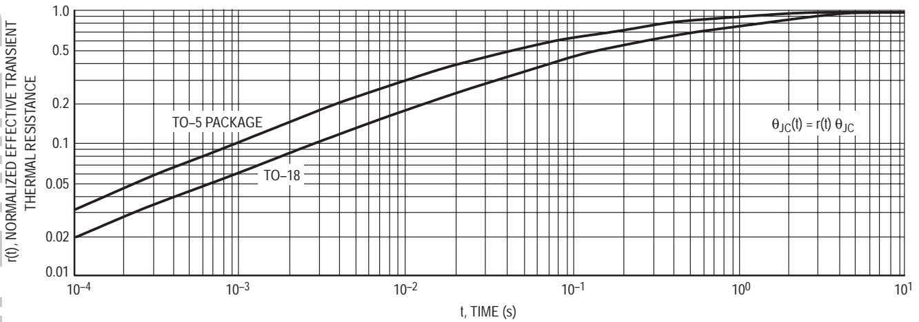
Figure 19. Thermal Resistance
